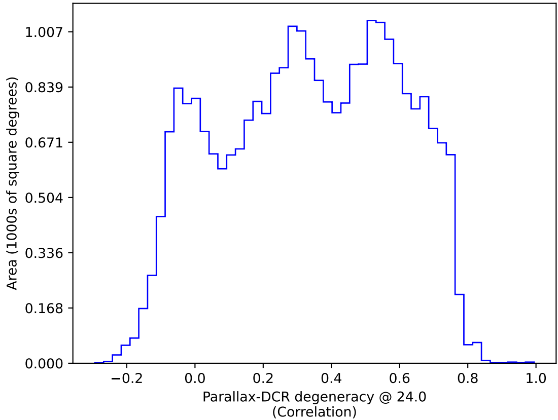
early_ss_template_fpextra3.0_v3.4_10yrs : Parallax-DCR degeneracy @ 24.0
