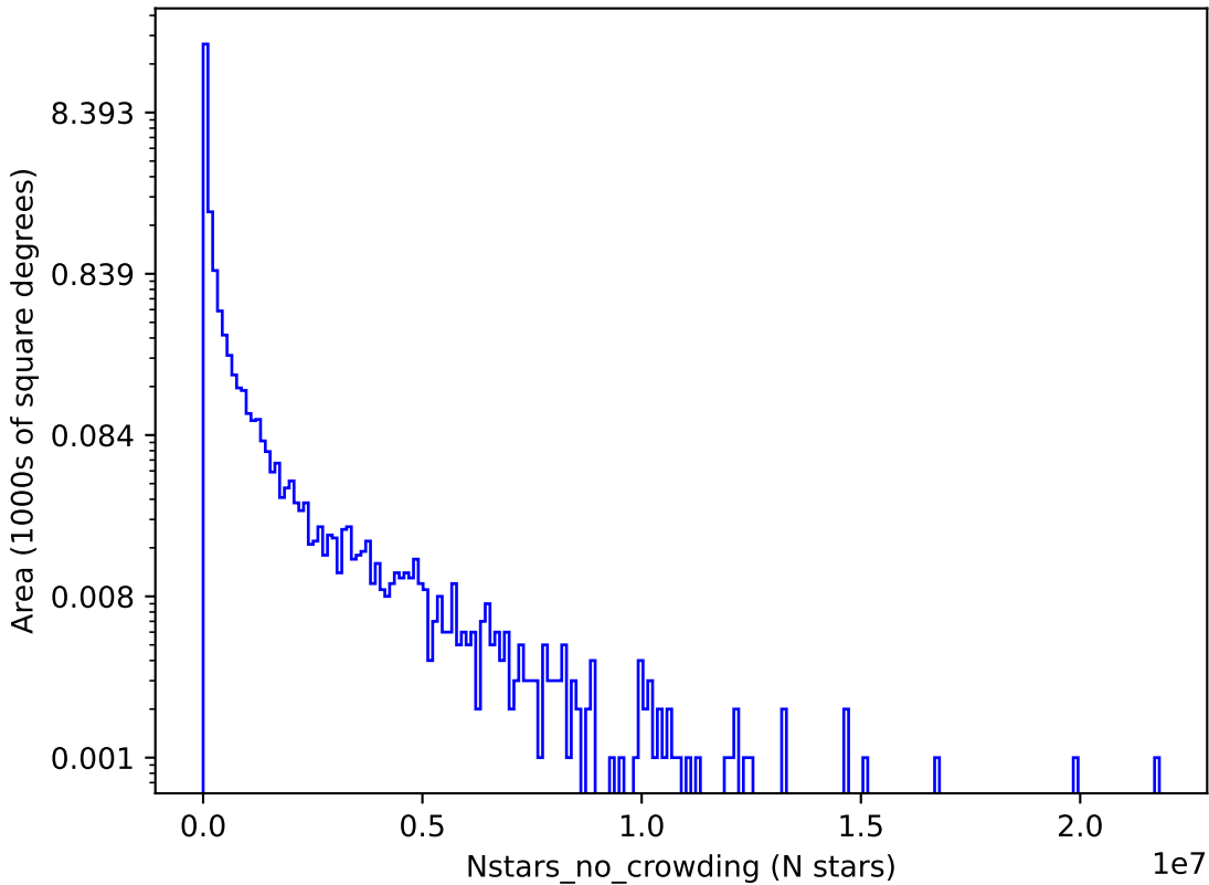
early_ss_template_fpextra3.0_v3.4_10yrs r: Nstars_no_crowding
