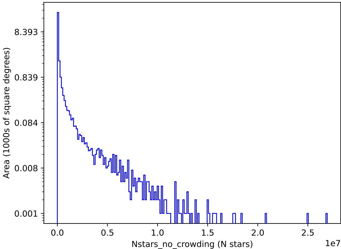
early_ss_template_fpextra3.0_v3.4_10yrs i: Nstars_no_crowding
