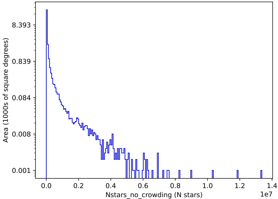
early_ss_template_fpextra3.0_v3.4_10yrs g: Nstars_no_crowding
