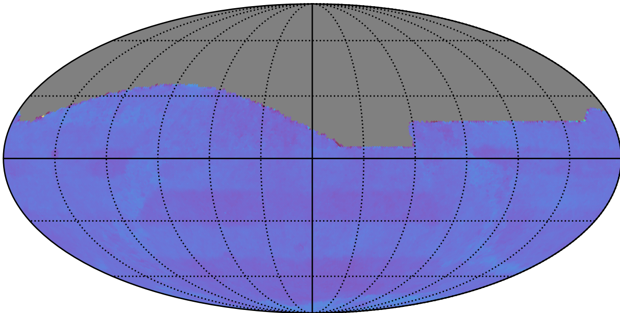
early_ss_template_fpextra3.0_v3.4_10yrs : Normalized Proper Motion Uncert @ 24.0
