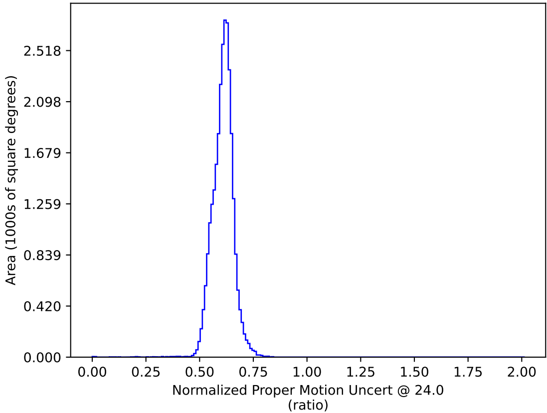
early_ss_template_fpextra3.0_v3.4_10yrs : Normalized Proper Motion Uncert @ 24.0
