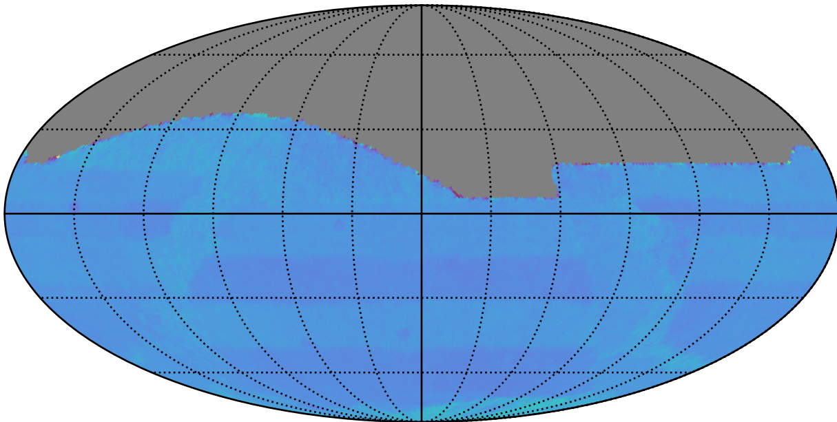
early_ss_template_fpextra3.0_v3.4_10yrs : Normalized Proper Motion Uncert @ 20.5
