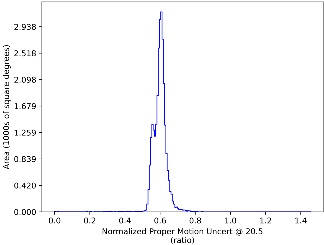
early_ss_template_fpextra3.0_v3.4_10yrs : Normalized Proper Motion Uncert @ 20.5
