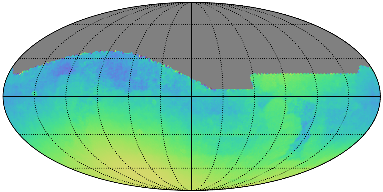
early_ss_template_fpextra3.0_v3.4_10yrs : Normalized Parallax Uncert @ 22.4
