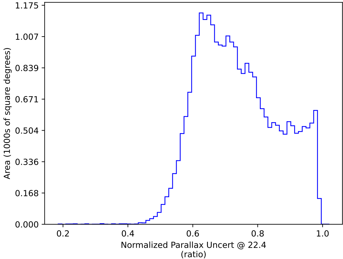
early_ss_template_fpextra3.0_v3.4_10yrs : Normalized Parallax Uncert @ 22.4
