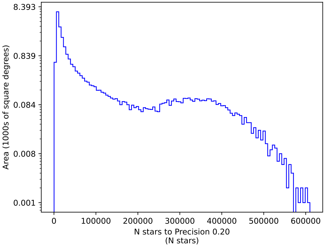
early_ss_template_fpextra3.0_v3.4_10yrs y: N stars to Precision 0.20
