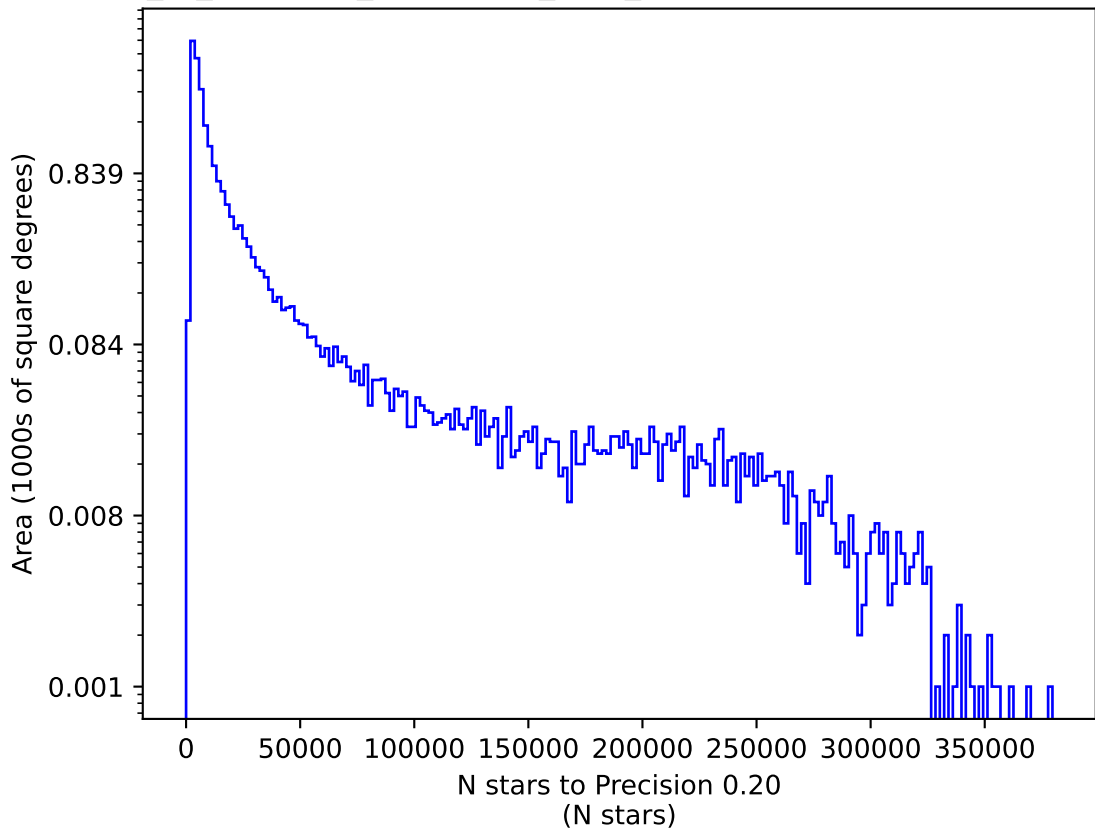
early_ss_template_fpextra3.0_v3.4_10yrs u: N stars to Precision 0.20
