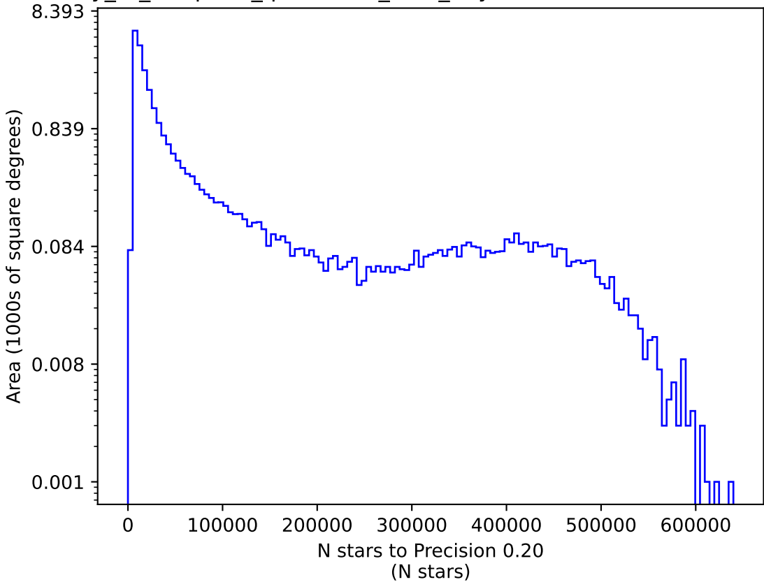
early_ss_template_fpextra3.0_v3.4_10yrs i: N stars to Precision 0.20
