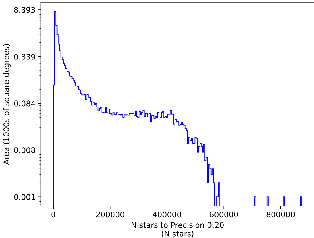
early_ss_template_fpextra3.0_v3.4_10yrs g: N stars to Precision 0.20
