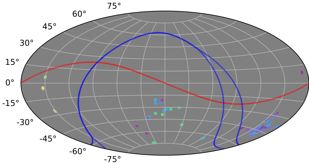
early_ss_template_fpextra3.0_v3.4_10yrs gi: LVDwarfs
