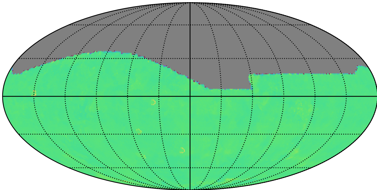
early_ss_template_fpextra3.0_v3.4_10yrs r: Kuiper rotTelPos
