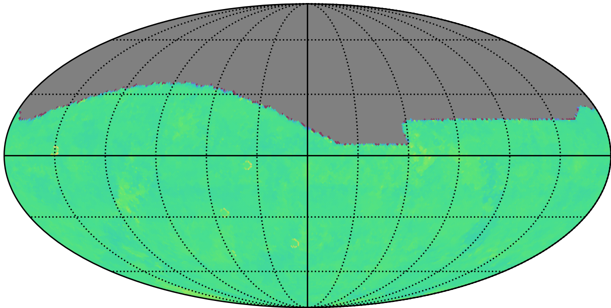
early_ss_template_fpextra3.0_v3.4_10yrs g: Kuiper rotTelPos
