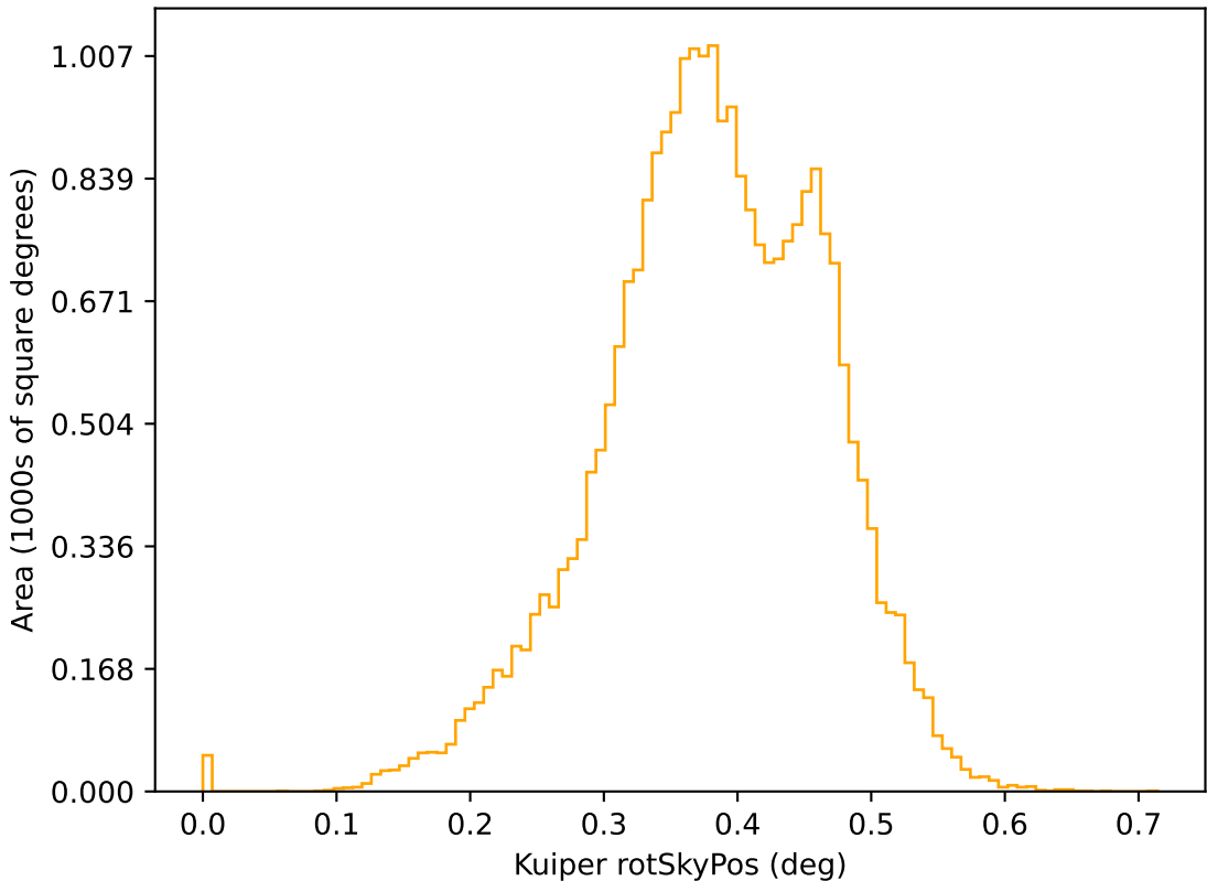
early_ss_template_fpextra3.0_v3.4_10yrs r: Kuiper rotSkyPos
