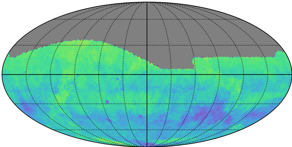
early_ss_template_fpextra3.0_v3.4_10yrs i: Kuiper rotSkyPos
