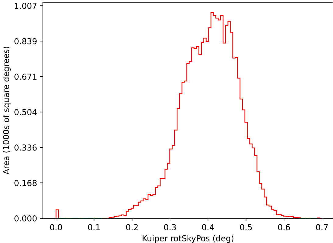
early_ss_template_fpextra3.0_v3.4_10yrs i: Kuiper rotSkyPos
