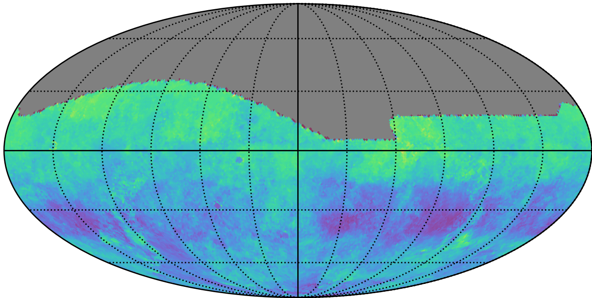
early_ss_template_fpextra3.0_v3.4_10yrs g: Kuiper rotSkyPos
