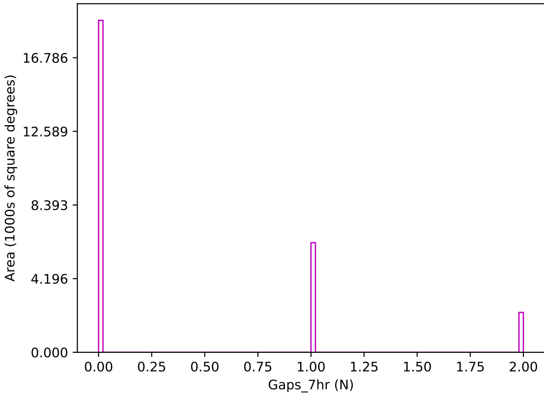
early_ss_template_fpextra3.0_v3.4_10yrs z band: Gaps_7hr
