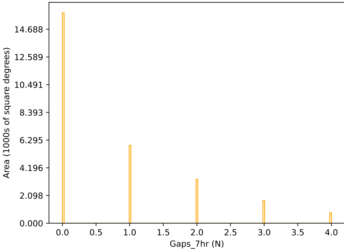
early_ss_template_fpextra3.0_v3.4_10yrs r band: Gaps_7hr
