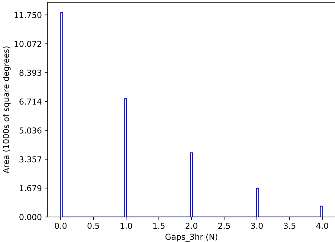
early_ss_template_fpextra3.0_v3.4_10yrs y band: Gaps_3hr
