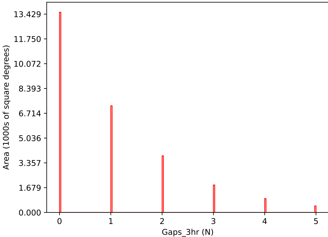
early_ss_template_fpextra3.0_v3.4_10yrs i band: Gaps_3hr
