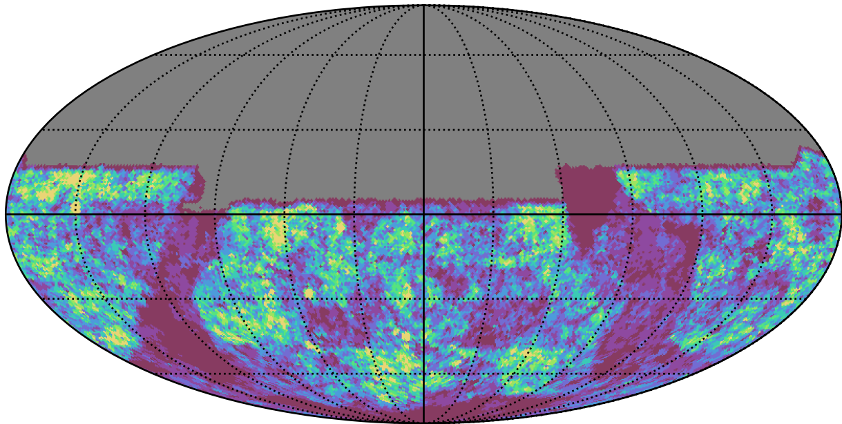
early_ss_template_fpextra3.0_v3.4_10yrs u band: Gaps_24hr
