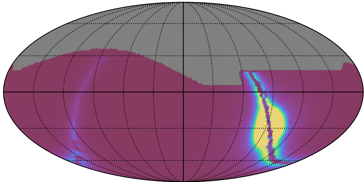
early_ss_template_fpextra3.0_v3.4_10yrs : GalplaneFootprintMetric_xray_binaries_map_Tau_73_0
