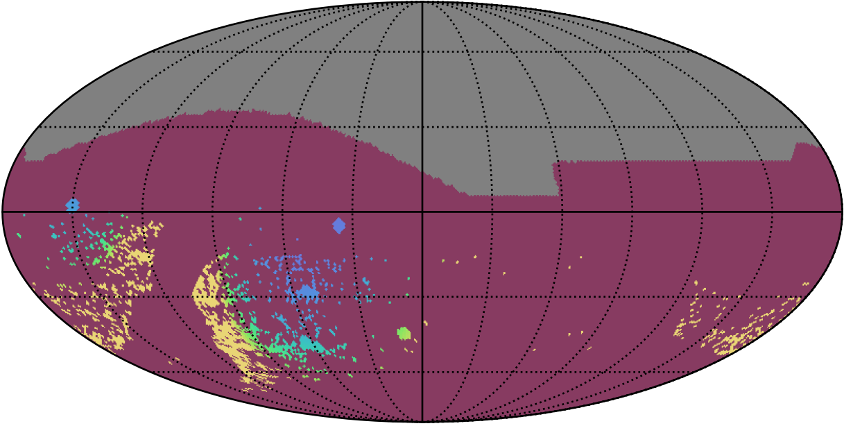
early_ss_template_fpextra3.0_v3.4_10yrs : GalplaneFootprintMetric_xray_binaries_map_Tau_5_0
