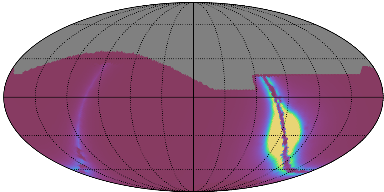
early_ss_template_fpextra3.0_v3.4_10yrs : GalplaneFootprintMetric_xray_binaries_map_Tau_46_5
