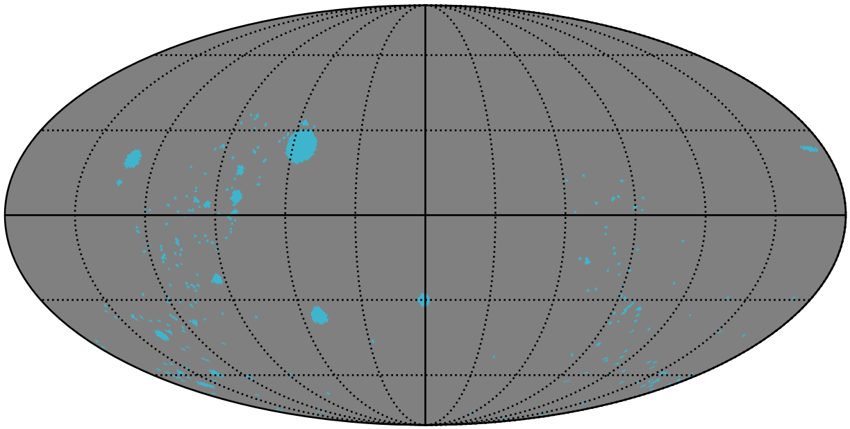
early_ss_template_fpextra3.0_v3.4_10yrs : GalplaneFootprintMetric_open_clusters_map_Tau_2_0
