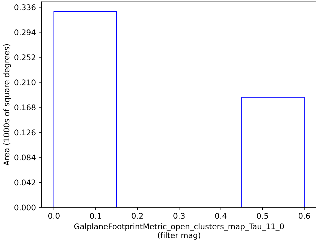
early_ss_template_fpextra3.0_v3.4_10yrs : GalplaneFootprintMetric_open_clusters_map_Tau_11_0
