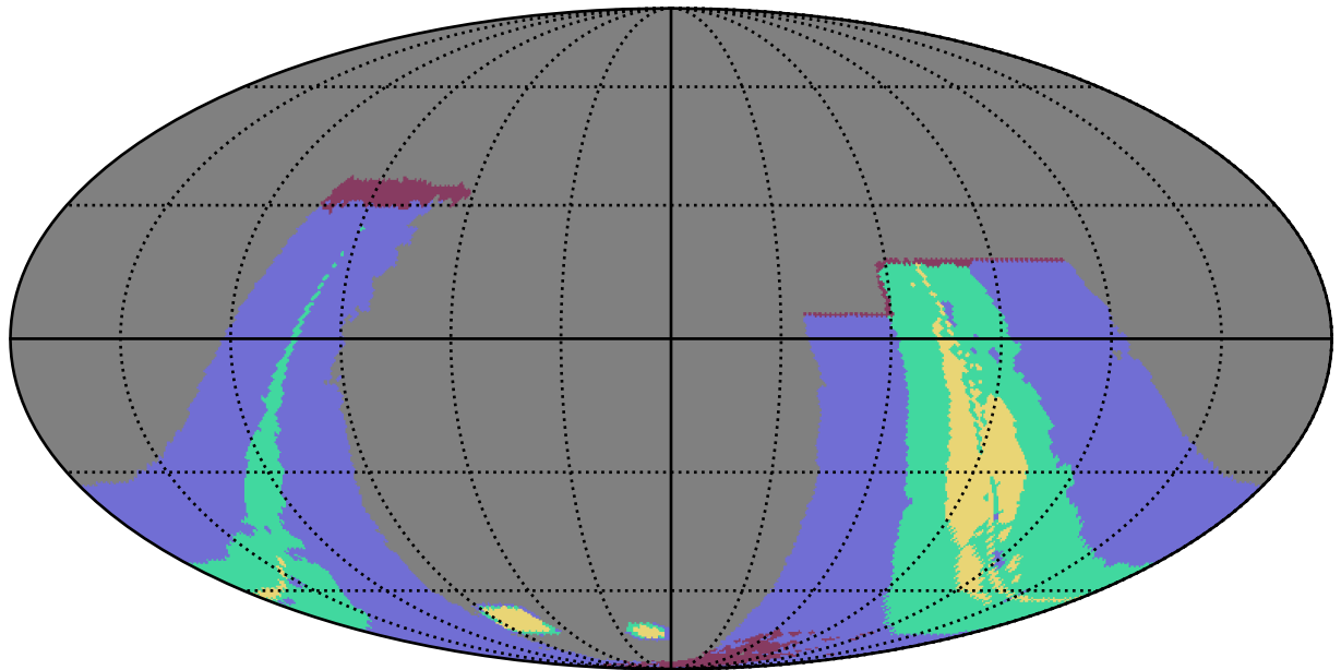
early_ss_template_fpextra3.0_v3.4_10yrs : GalplaneFootprintMetric_galactic_plane_map_Tau_73_0
