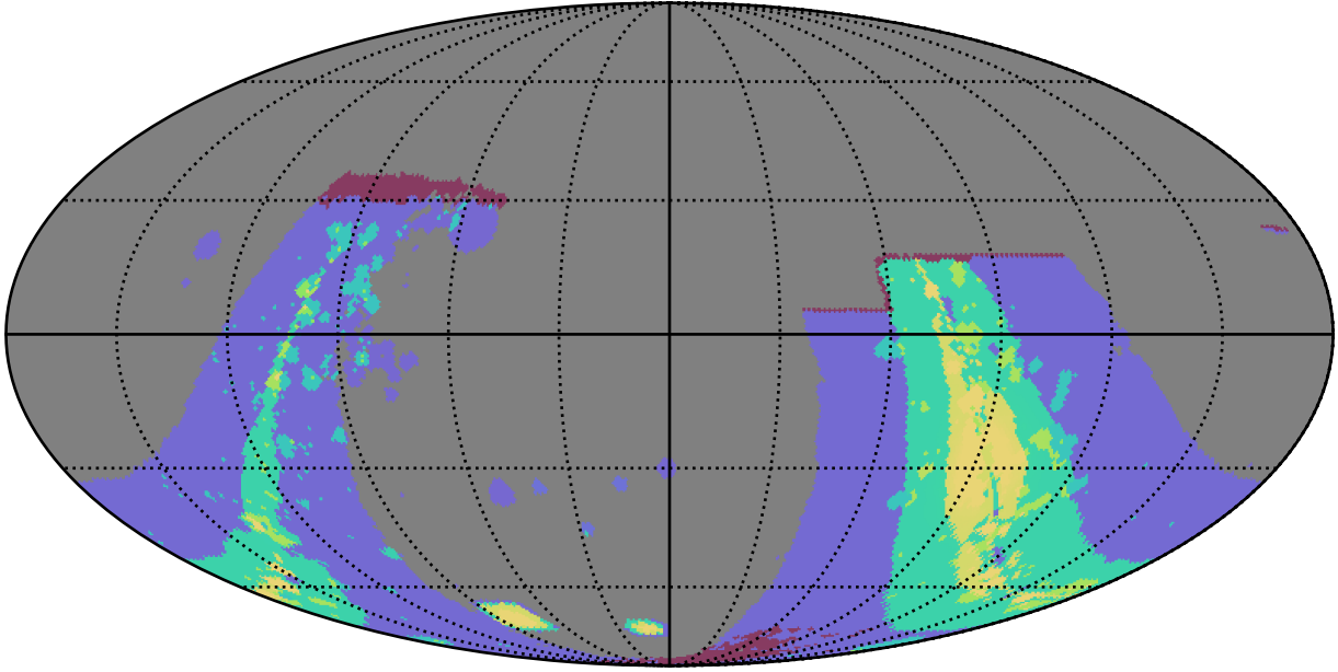
early_ss_template_fpextra3.0_v3.4_10yrs : GalplaneFootprintMetric_combined_map_Tau_73_0
