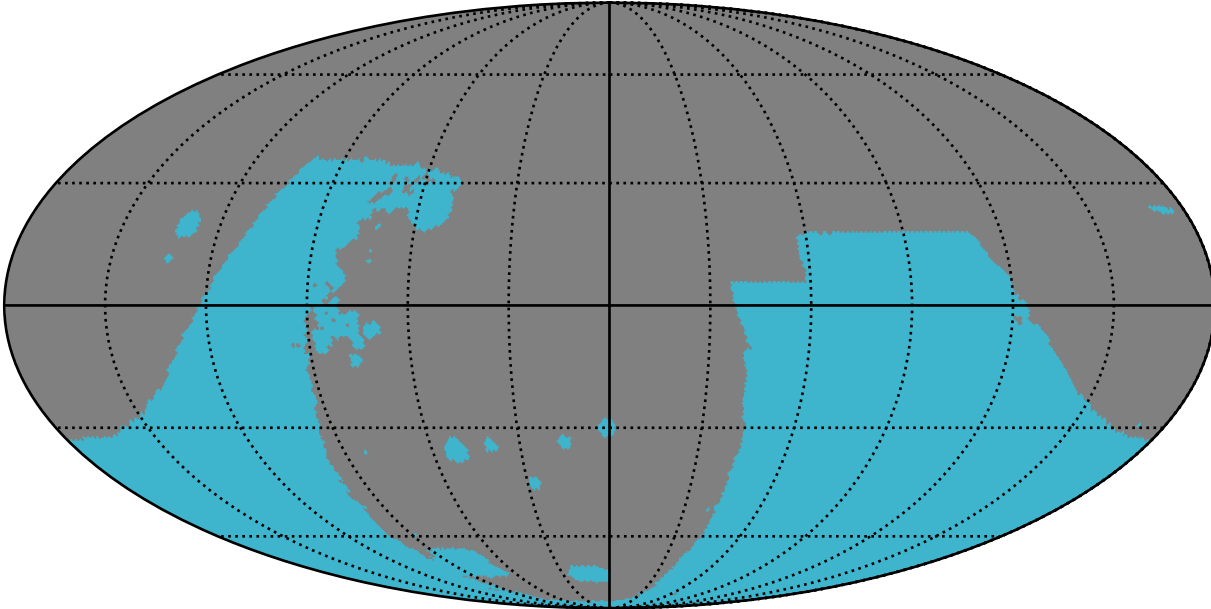
early_ss_template_fpextra3.0_v3.4_10yrs : GalplaneFootprintMetric_combined_map_Tau_2_0
