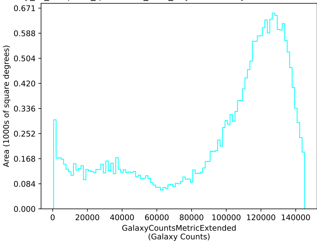
early_ss_template_fpextra3.0_v3.4_10yrs u: GalaxyCountsMetricExtended
