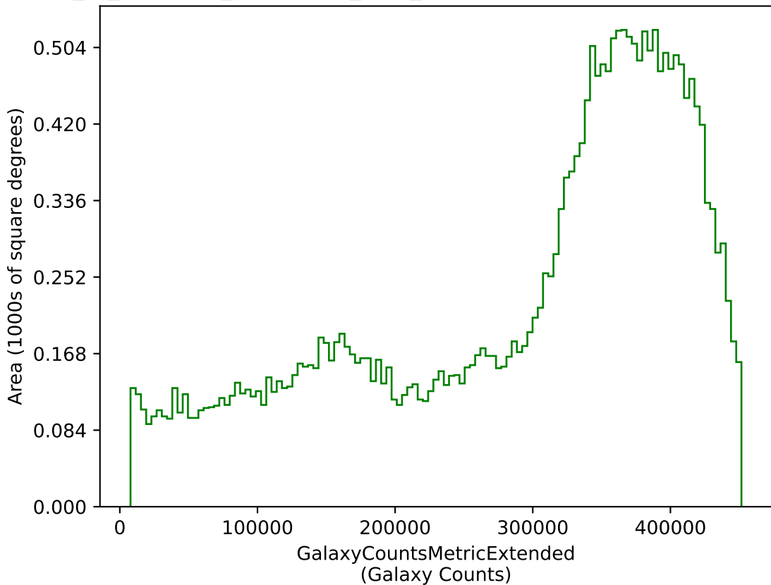
early_ss_template_fpextra3.0_v3.4_10yrs g: GalaxyCountsMetricExtended
