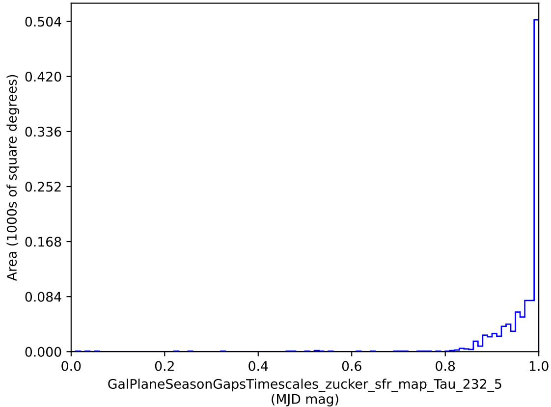
early_ss_template_fpextra3.0_v3.4_10yrs : GalPlaneSeasonGapsTimescales_zucker_sfr_map_Tau_232_5
