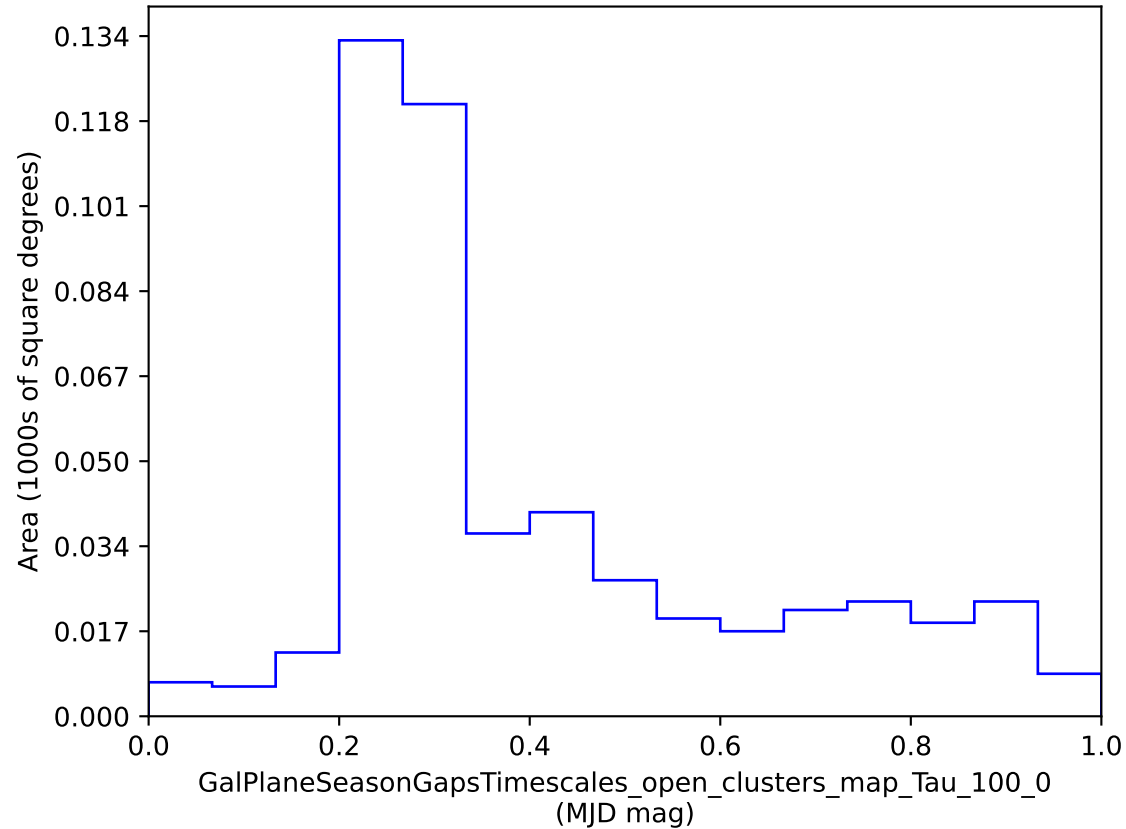
early_ss_template_fpextra3.0_v3.4_10yrs : GalPlaneSeasonGapsTimescales_open_clusters_map_Tau_100_0
