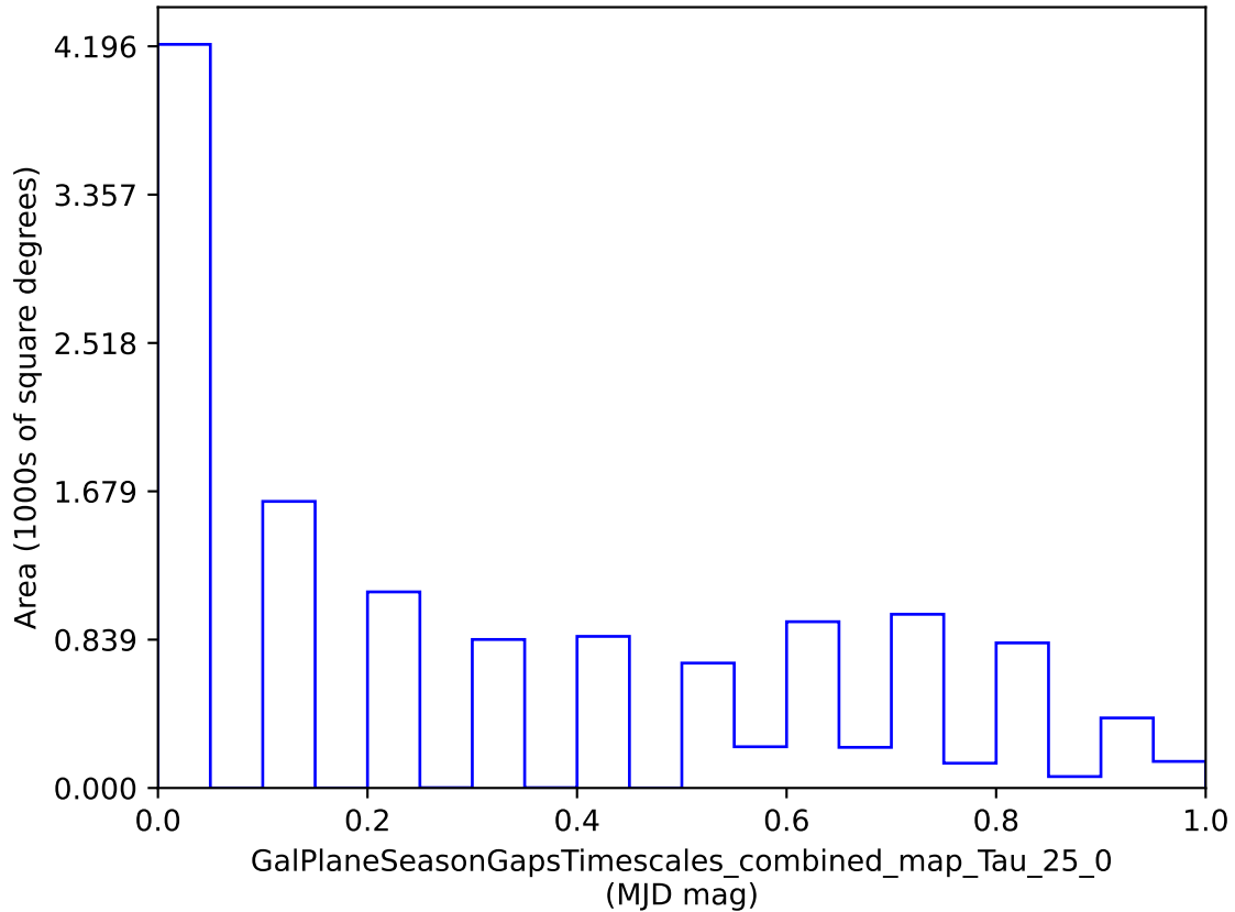
early_ss_template_fpextra3.0_v3.4_10yrs : GalPlaneSeasonGapsTimescales_combined_map_Tau_25_0
