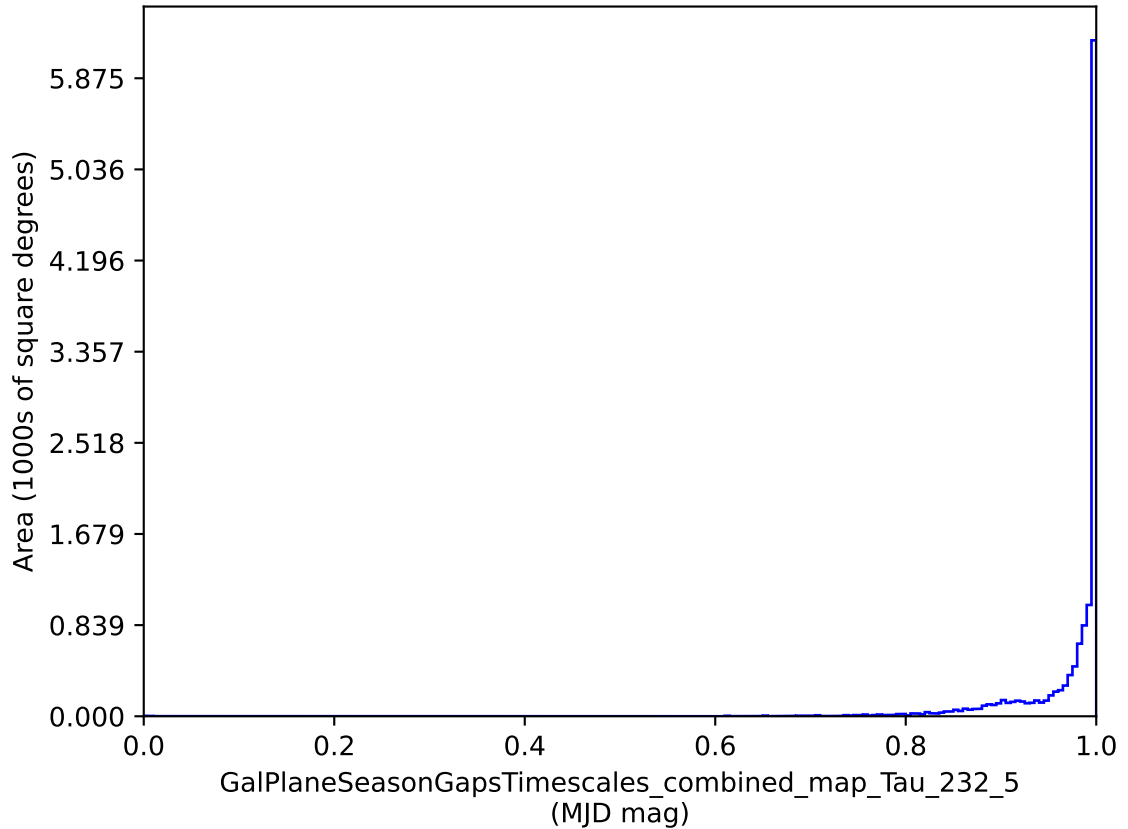
early_ss_template_fpextra3.0_v3.4_10yrs : GalPlaneSeasonGapsTimescales_combined_map_Tau_232_5
