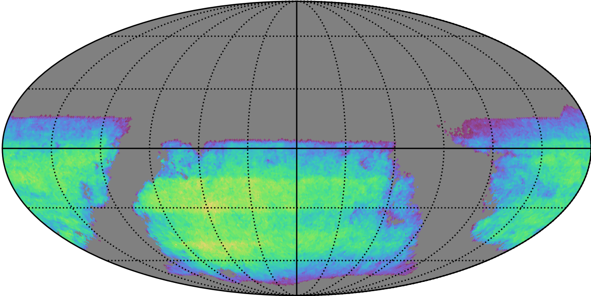
early_ss_template_fpextra3.0_v3.4_10yrs i band non-DD year 9: ExgalM5WithCuts
