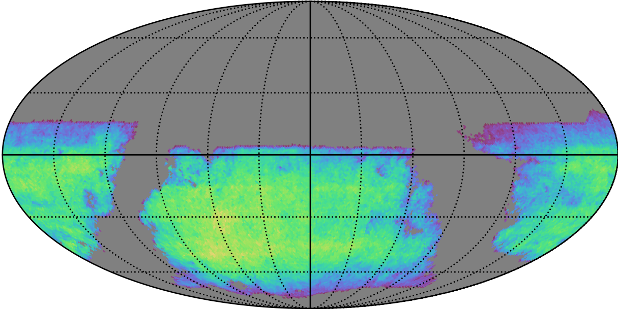
early_ss_template_fpextra3.0_v3.4_10yrs i band non-DD year 8: ExgalM5WithCuts
