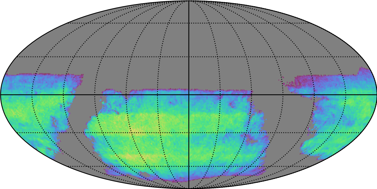
early_ss_template_fpextra3.0_v3.4_10yrs i band non-DD year 7: ExgalM5WithCuts
