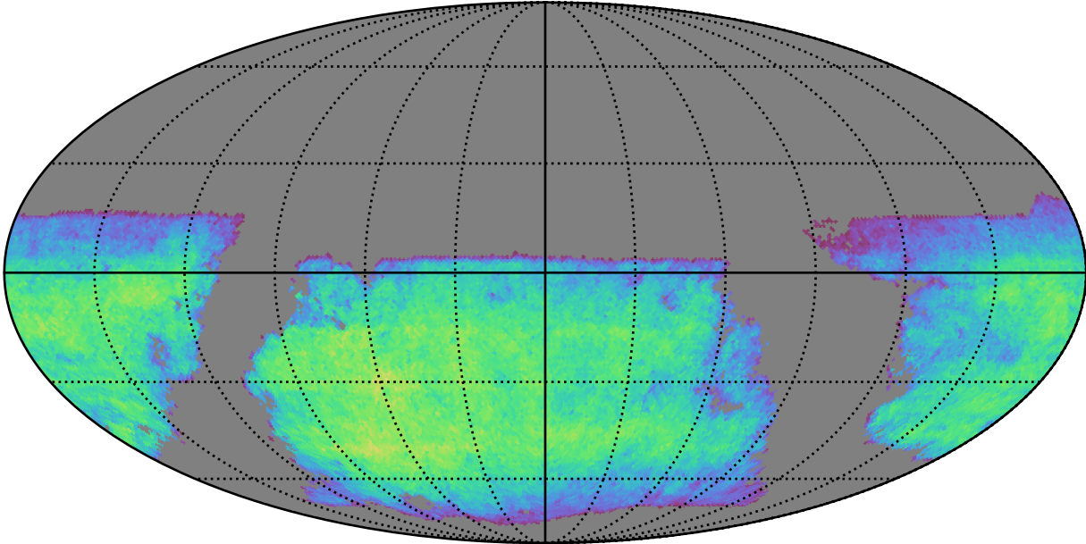
early_ss_template_fpextra3.0_v3.4_10yrs i band non-DD year 6: ExgalM5WithCuts
