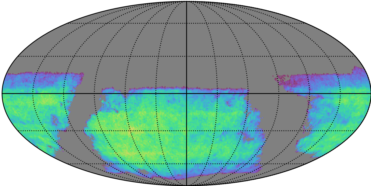
early_ss_template_fpextra3.0_v3.4_10yrs i band non-DD year 4: ExgalM5WithCuts
