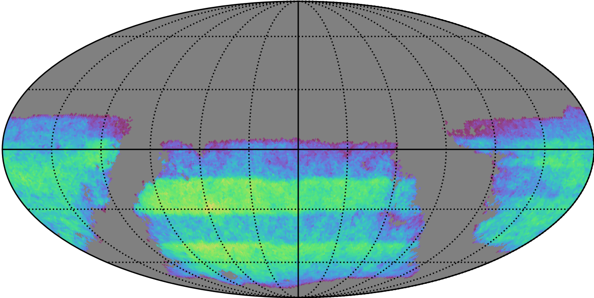
early_ss_template_fpextra3.0_v3.4_10yrs i band non-DD year 3: ExgalM5WithCuts
