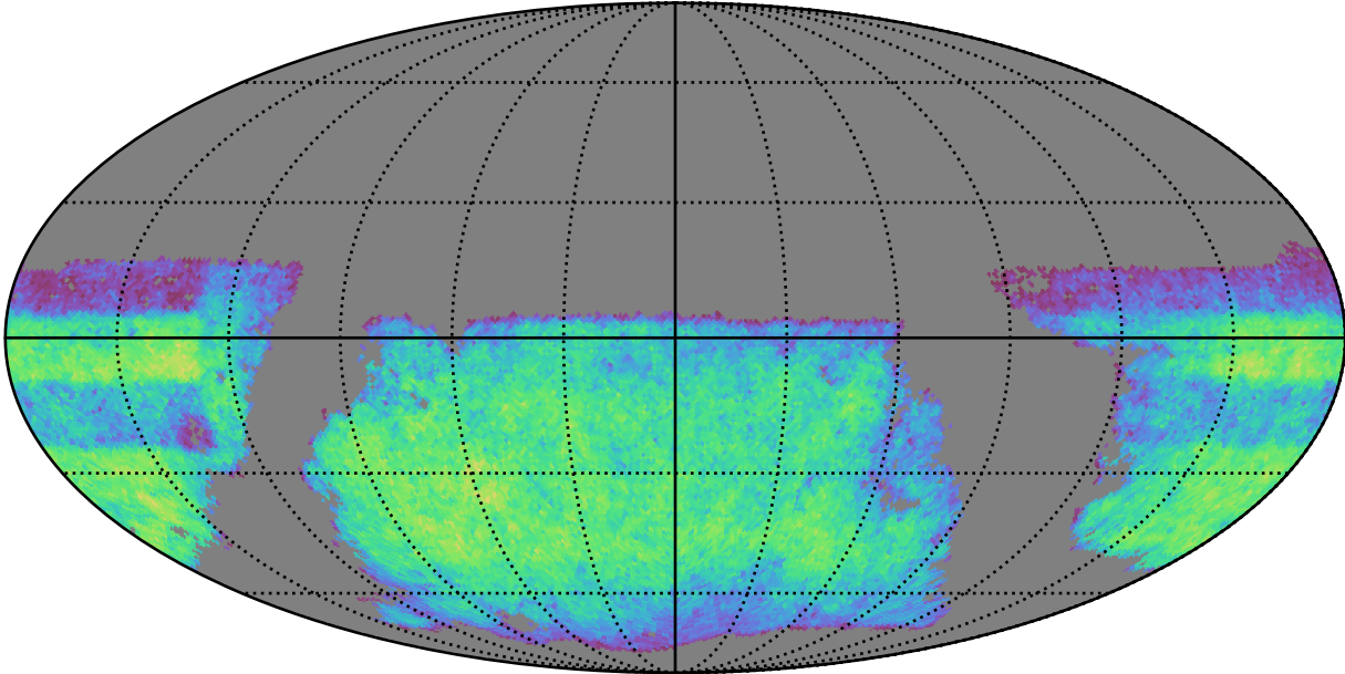
early_ss_template_fpextra3.0_v3.4_10yrs i band non-DD year 2: ExgalM5WithCuts
