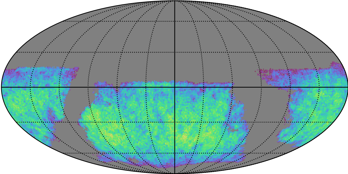
early_ss_template_fpextra3.0_v3.4_10yrs i band non-DD year 1: ExgalM5WithCuts
