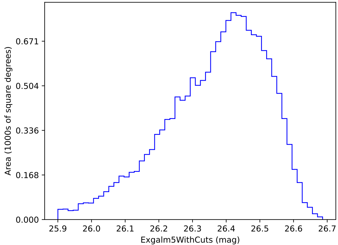
early_ss_template_fpextra3.0_v3.4_10yrs i band non-DD year 10: ExgalM5WithCuts
