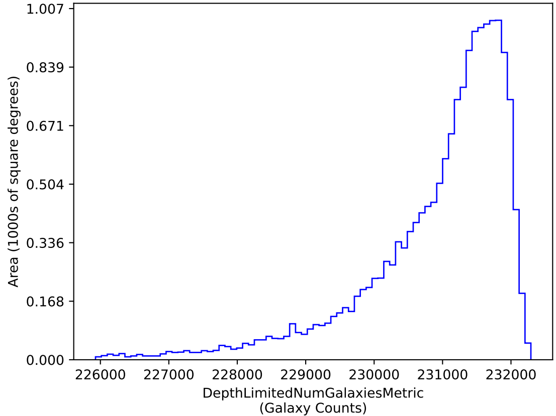
early_ss_template_fpextra3.0_v3.4_10yrs i band galaxies non-DD: DepthLimitedNumGalaxiesMetric
